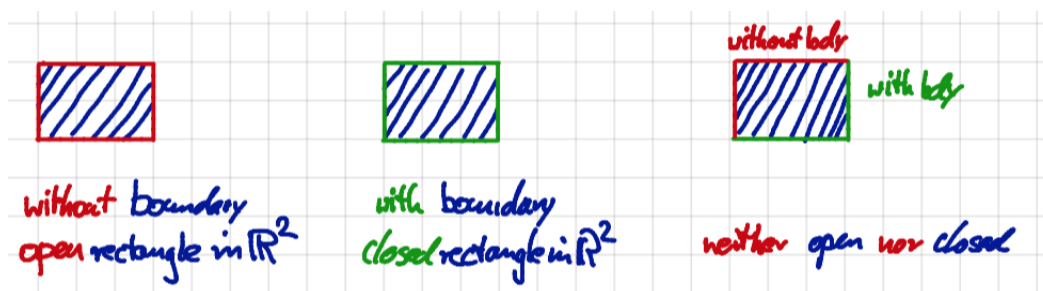
Figure 2.2: Examples of subsets in \mathbb{R}^2 .
