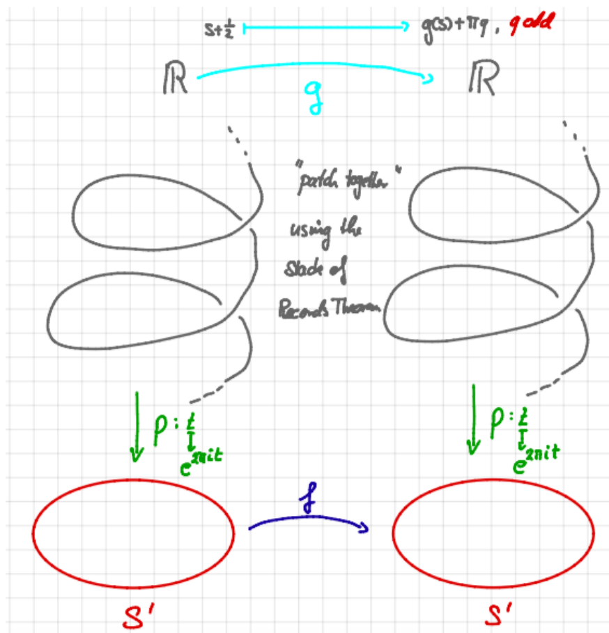
Figure 12.4: We think of \mathbb{R} lying as a spiral above S^1 . That makes it easier to imagine how we lift f to a map g , first by local lifts which then are patched together.
