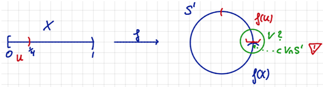
Figure 2.5: Wrapping the interval around the circle via f is a bijection, but not a homeomorphism, since f(U) may not be open in S^1 .
