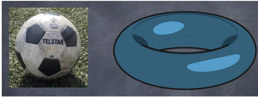
Figure 1.2: Two examples of smooth manifolds: a sphere and a torus.
