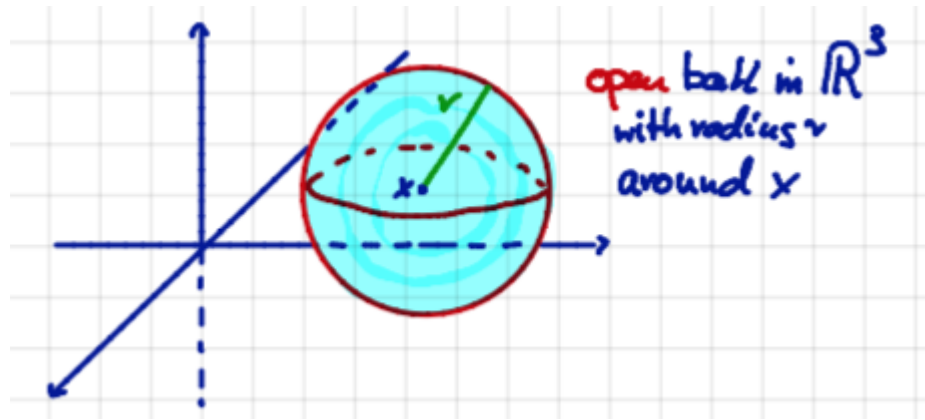
Figure 2.1: An open ball in \mathbb{R}^3 .
