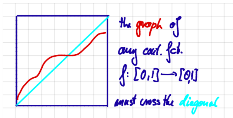
Figure 11.3: In dimension one this is the Intermediate Value Theorem. The graph has to cross the diagonal which consists of fixed points of f .
