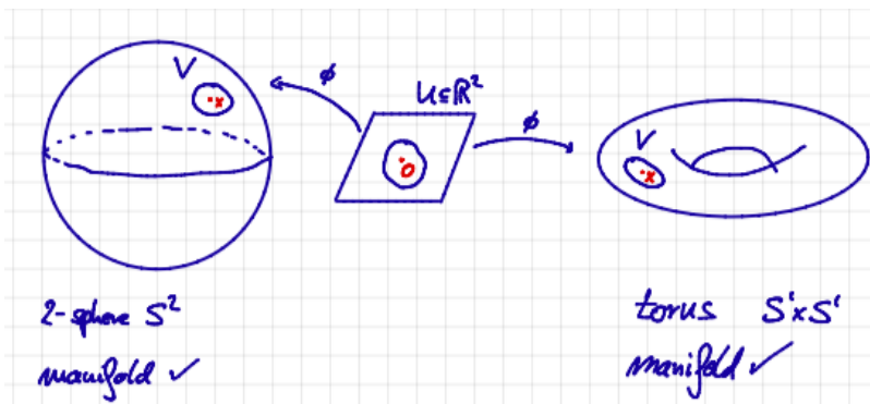
Figure 2.9: Points on S^2 and on T^2 have both open neighborhoods diffeomorphic to open subsets in \mathbb{R}^2 . However, S^2 and T^2 have different global properties.
