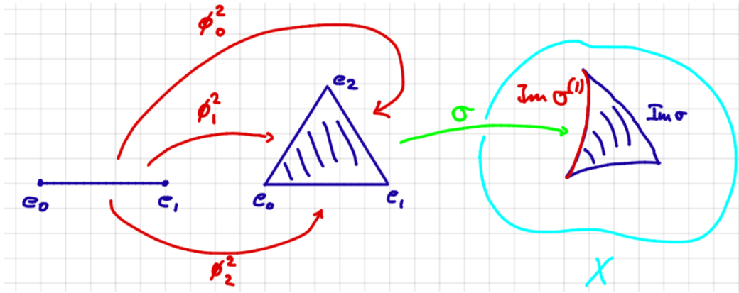
Figure 18.4: The face maps from the one-dimensional simplex into the two-dimensional one. There are three maps corresponding to the three edges of \Delta^2 . Then \sigma maps the simplices to X .
