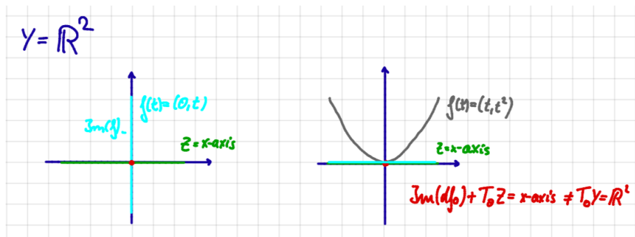
Figure 6.1: On the left, f is transverse to the x -axis, since \text{Im}(df_0) and T_0Z span all of T_0Y = \mathbb{R}^2 . On the right, however, f is not transverse to Z , since both \text{Im}(df_0) and T_0Z span the same one-dimensional subspace.
