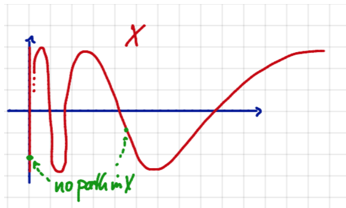
Figure 2.7: A connected but not path-connected space.
